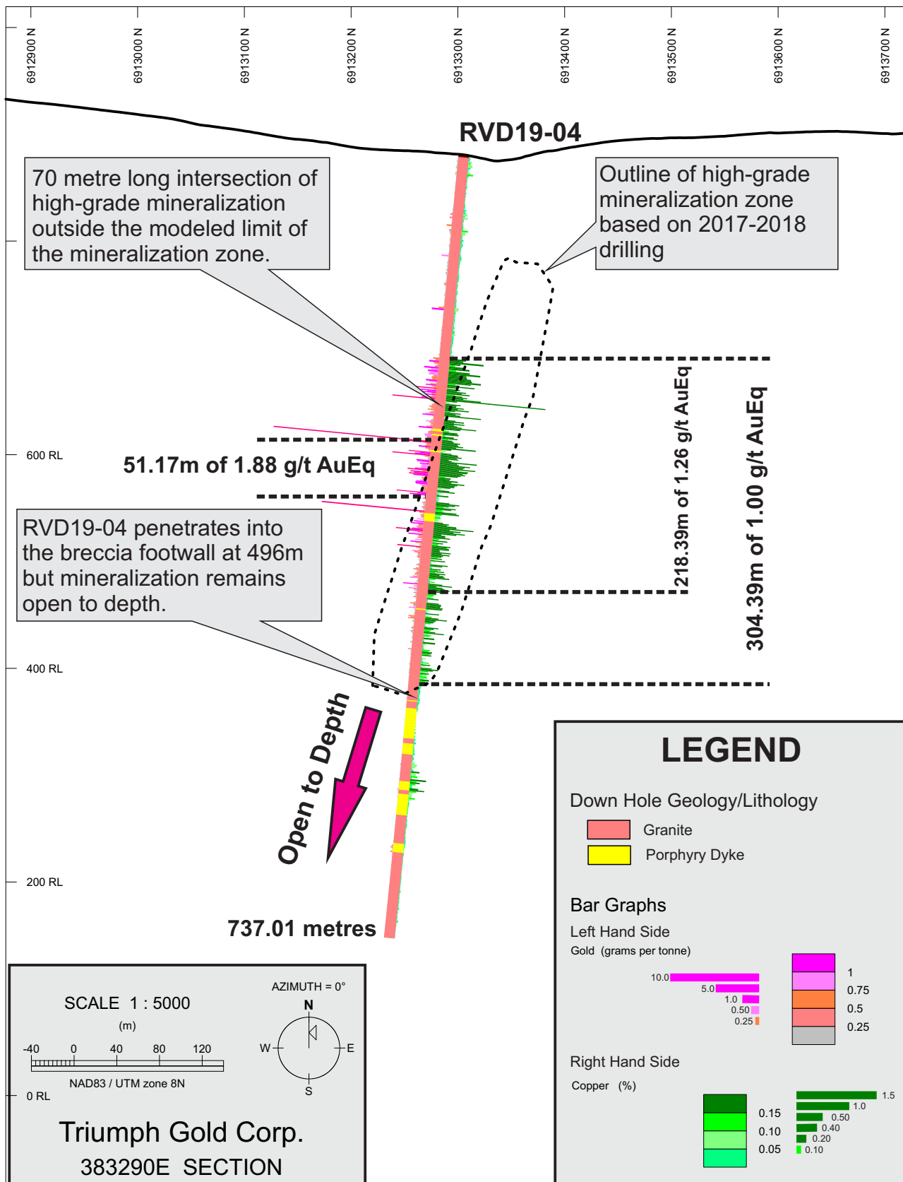
Figure 2 West Facing Cross Section
